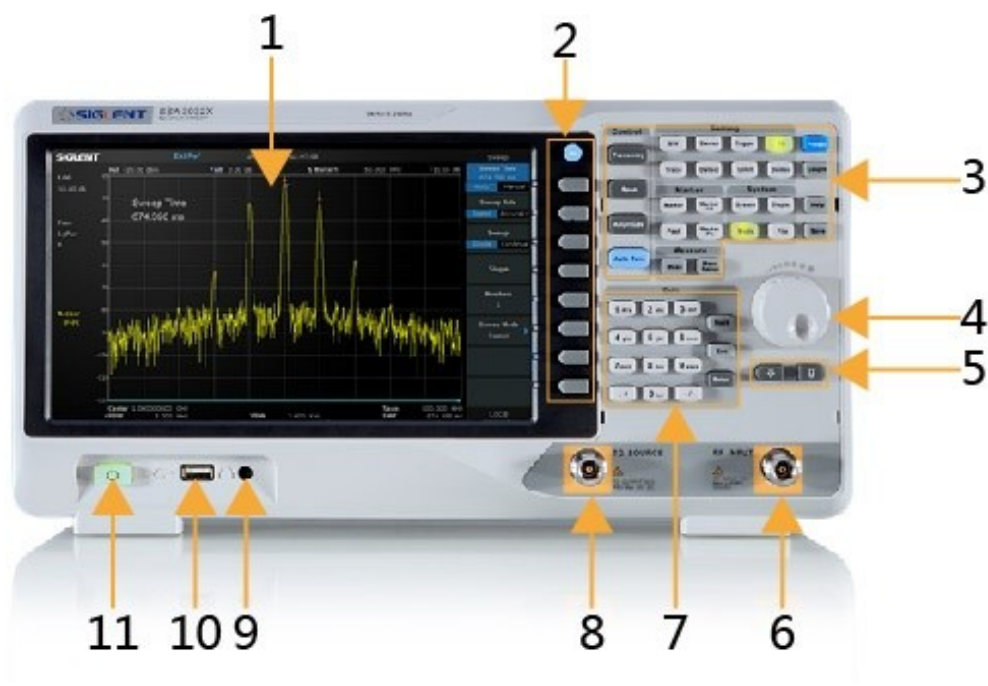
Figure 1-6 The Front Panel
