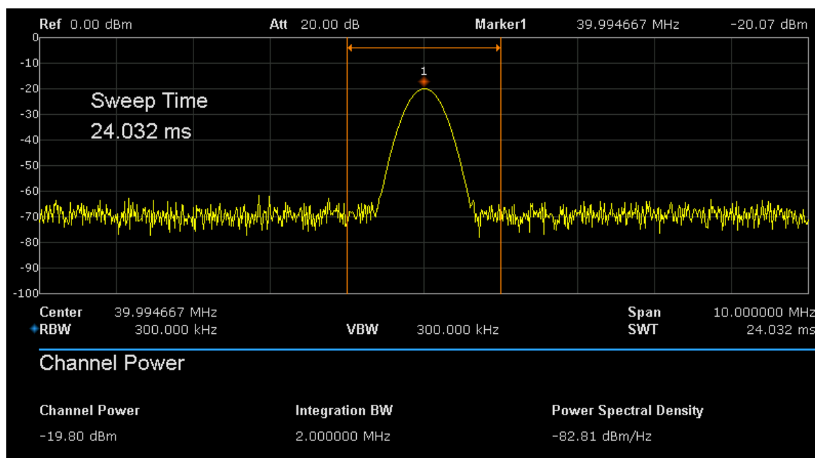
Figure 2-9 Channel Power
