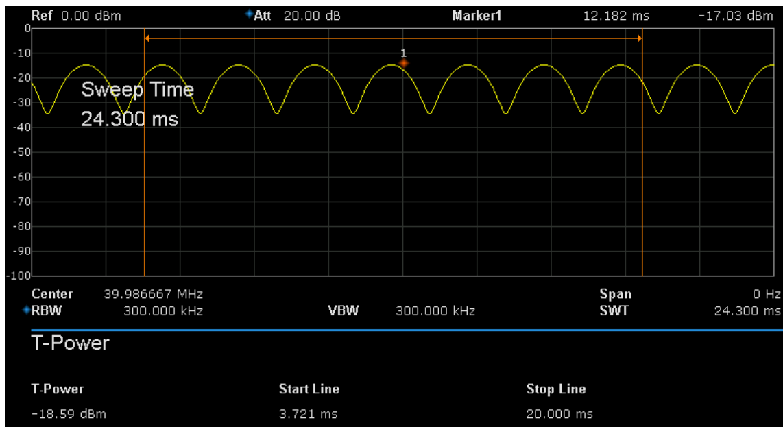
Figure 2-12 T-Power
