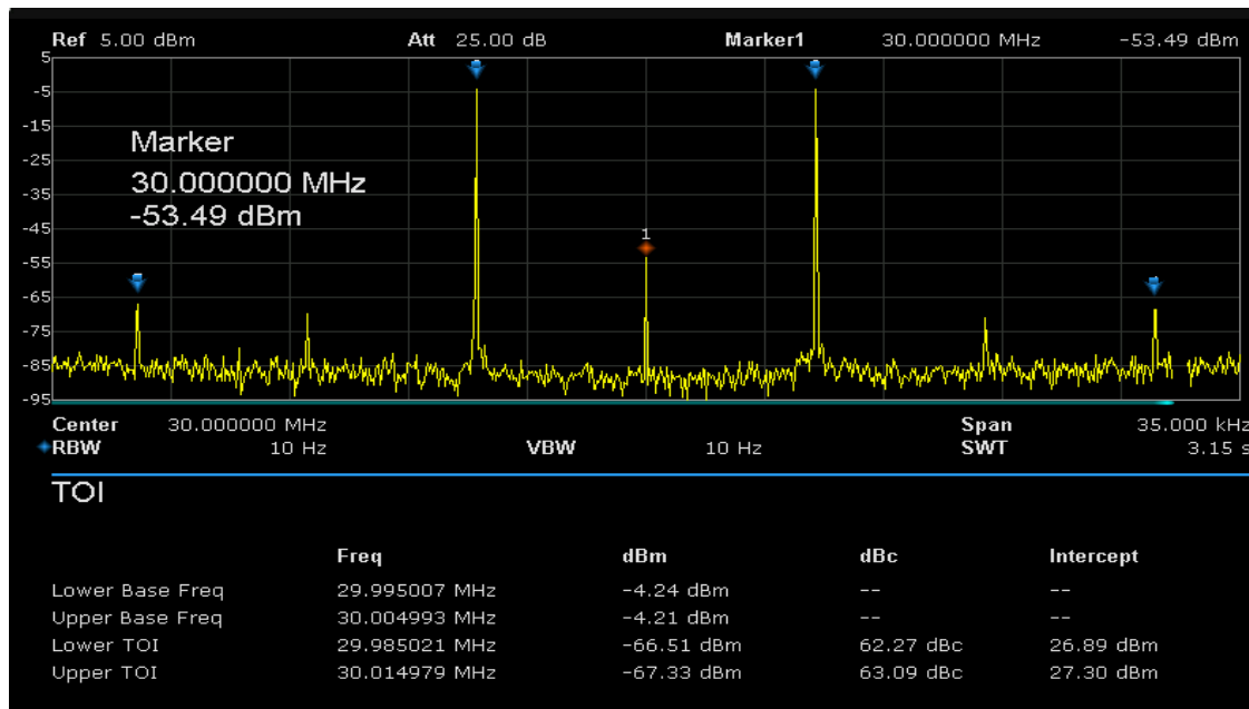
Figure 2-13 TOI
