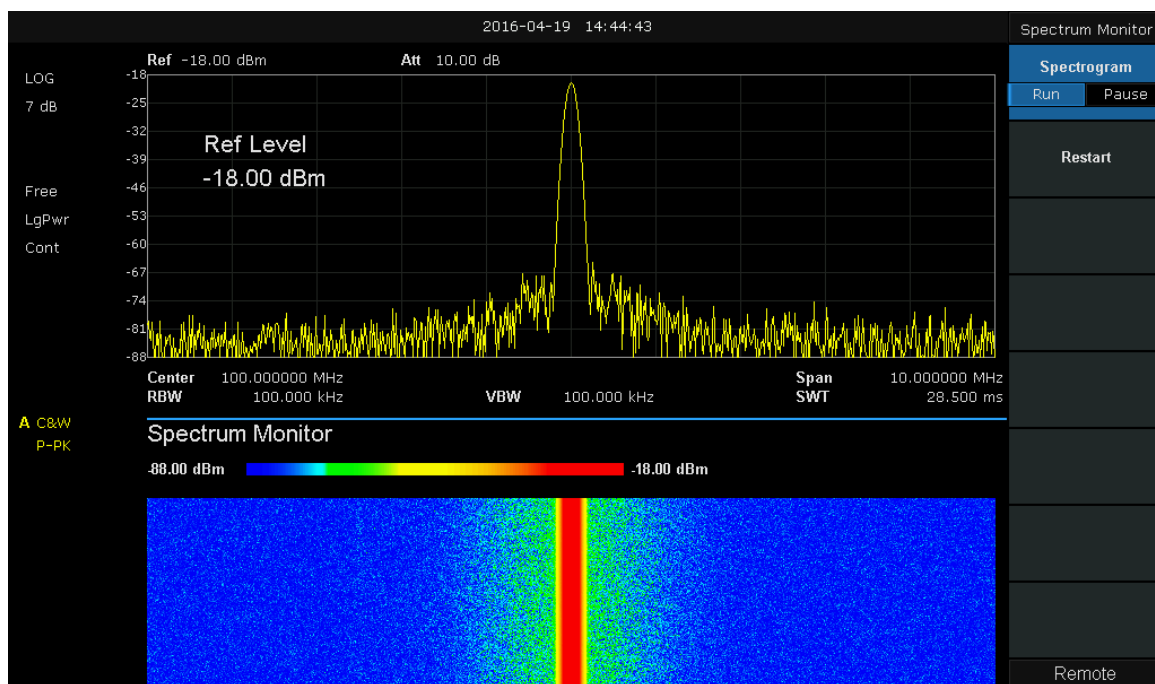
Figure 2-14 Spectrum Monitor
