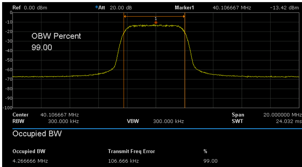
Figure 2-11 OBW
