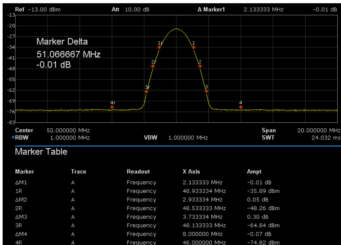
Figure 2-7 Marker table
