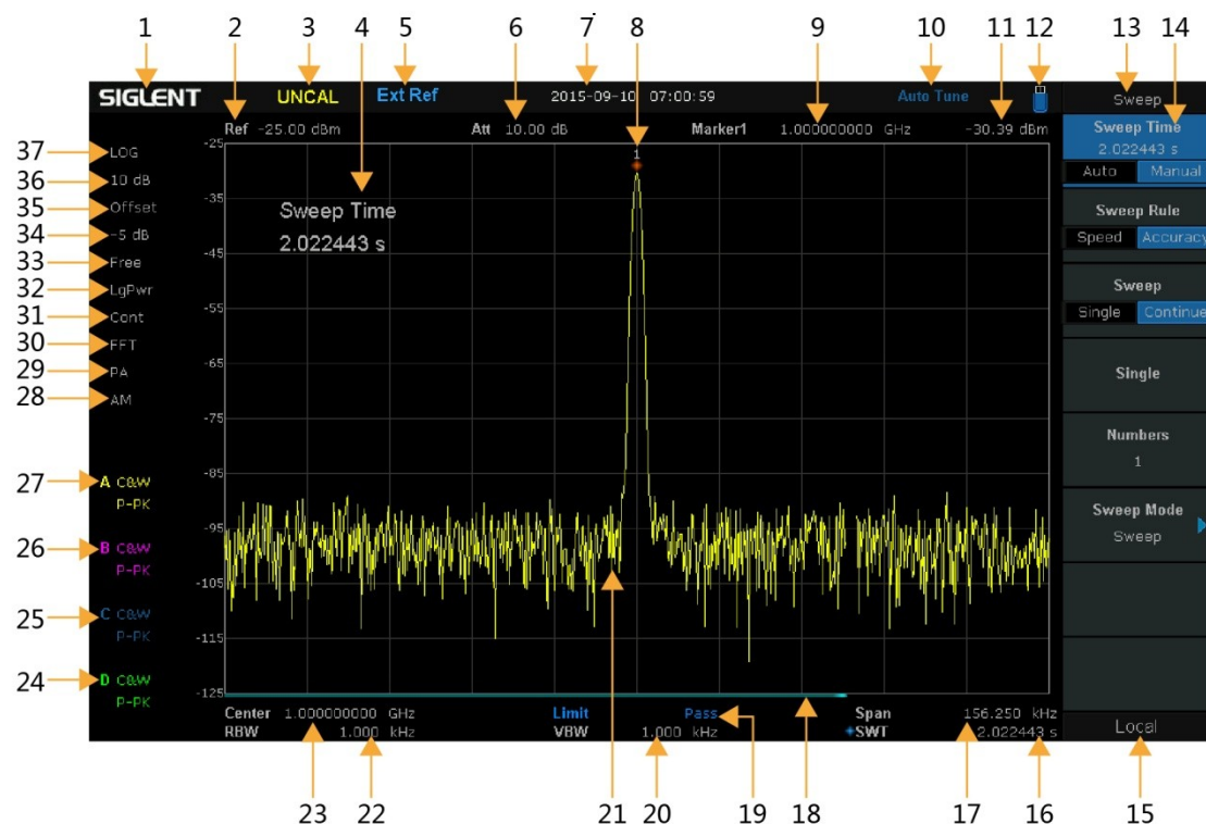
Figure 1-11 User Interface
